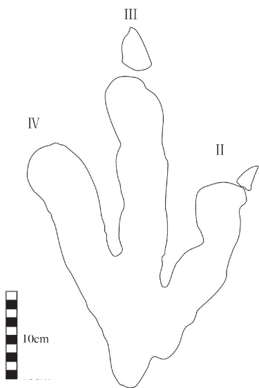
Fig. 3 Outline drawing of Changpeipus carbonicus (IVPP V2472.2)
