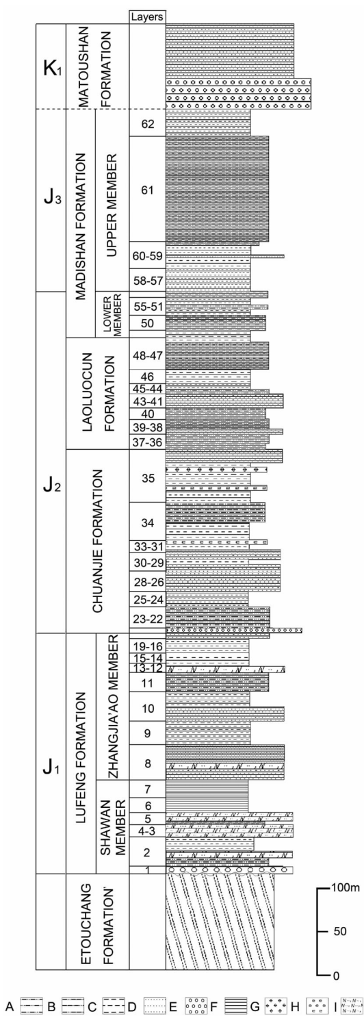
Fig. 2 Stratigraphic columns of the Jurassic strata of the Lufeng section (emended from Chen et al, 2004) A—pelitic siltstone;B—sandy mudstone;C—mudstone; D—sandstone;E—conglomerate;F—shale;G—orthomicrite; H—orthomicrite containing fossils;I—arkose
